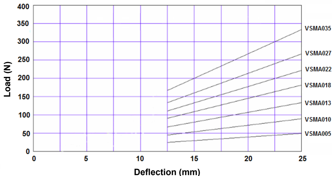
Load Deflection Characteristics
